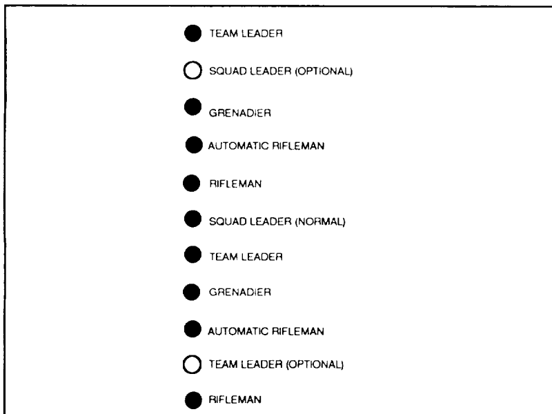
Figure 2-9. Squad file.
